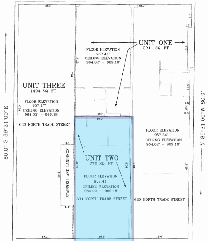
SECOND FLOOR
